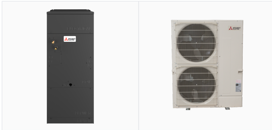
INDOOR Unit ... PVA-AA36NL OUTDOOR Unit ... PUZ-AK36NL
