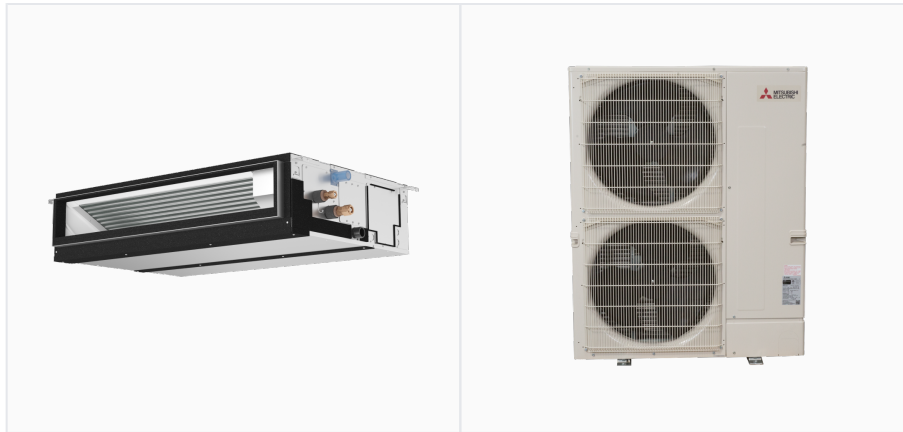
INDOOR Unit ... PEAD-AA36NL OUTDOOR Unit ... PUZ-AK36NL
