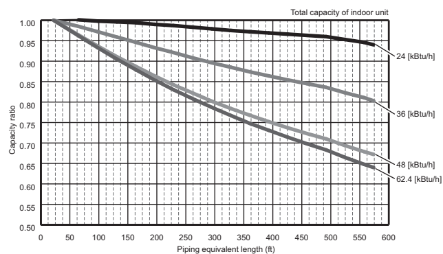
MXZ-SM48NL-U1, MXZ-SM48NLHZ-U1
