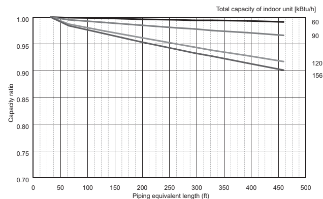
MXZ-SM120TL-U1
