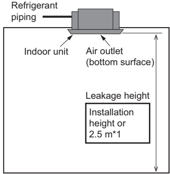
(5) Leakage height for ceiling concealed indoor unit
