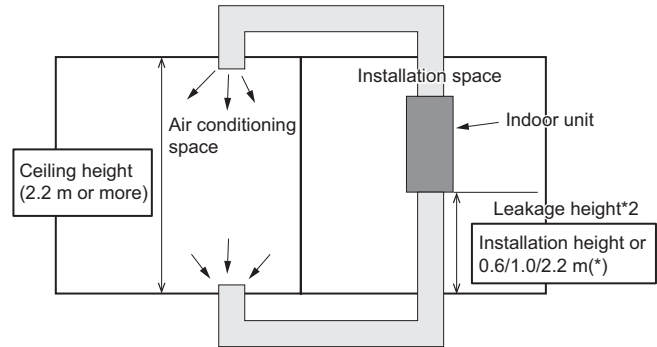
(4) Leakage height for vertical concealed indoor unit
