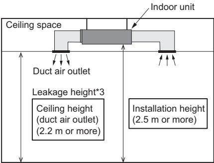
(5) Leakage height for ceiling concealed indoor unit
