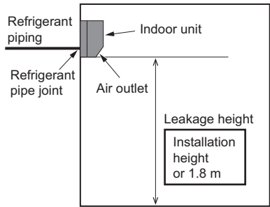
(1) Leakage height for wall-mounted indoor unit
