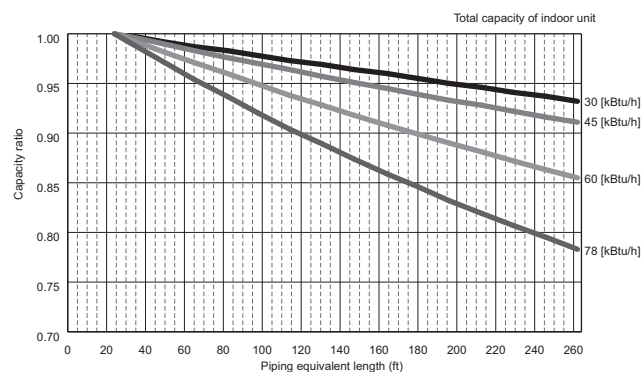
MXZ-SM60NL-U1, MXZ-SM60NLHZ-U1
