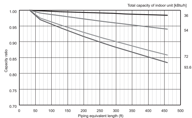
MXZ-SM72TL-U1
