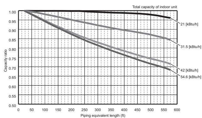
MXZ-SM60NL-U1, MXZ-SM60NLHZ-U1
