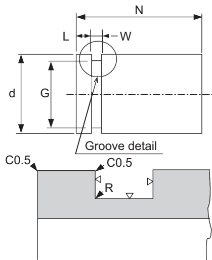
Groove specifications
