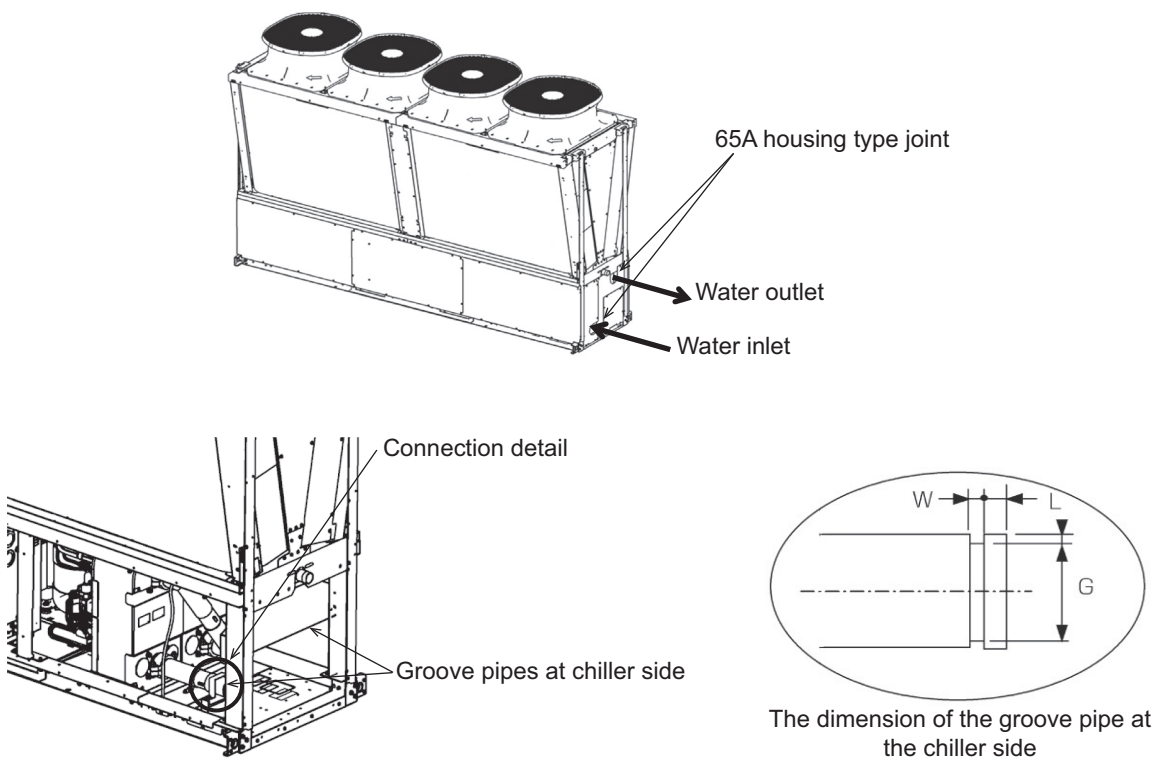
Groove specifications
