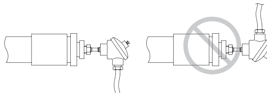
Horizontal installation
